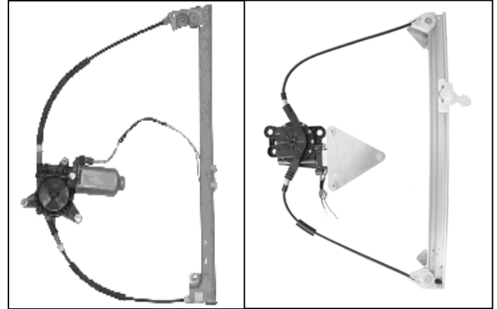
Elevavinas original Oem window regulator
