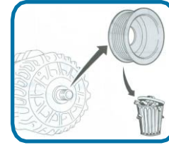
ANTI-VIBRATION KIT composed of crankshaft pulley Ref. 17-1325 and alternator pulley Ref. 30-1306 OEM → BMW: 11238593226
