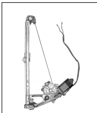
Elevalunas original – lève-vitre original – oem window regulator – levandator de vidro original
