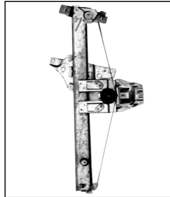
Elevavinas original – lève-vitre original – oem window regulator – levandator de vidro original
