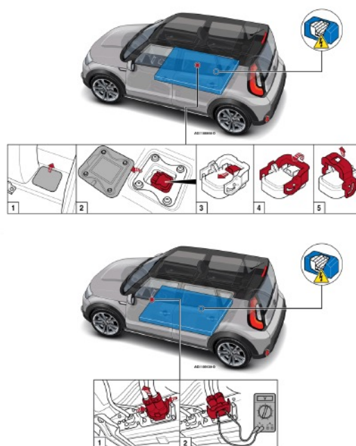
Figure 4. Location of the batteries in the Soul III.
