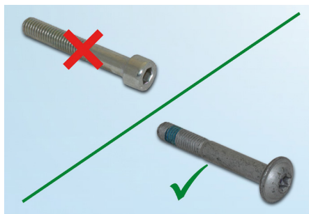
Figur 3: skruer
