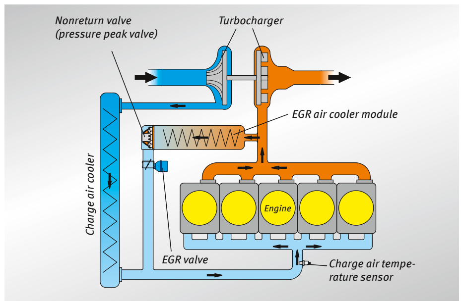
Diagram of the cooled exhaust gas return system
