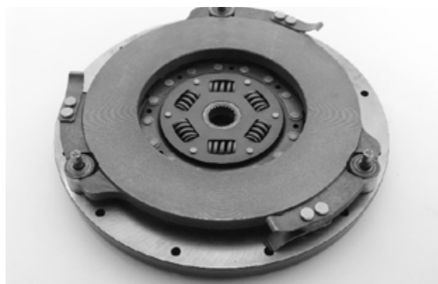
Fit intermediate plate. Note direction of release straps.
