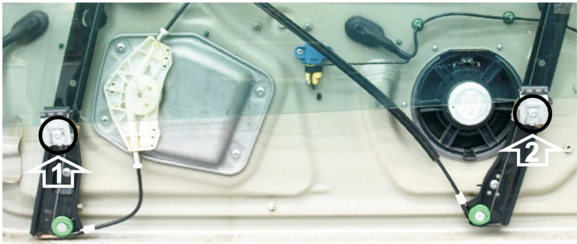
POWER WINDOW LEFT ORIGINAL
