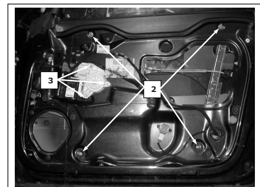
Porta lato destro, Portière avant droite, Right front door, Puerta lado derecho, Vorne rechte Tür, Porta frente diresita, Sag on kapi, πόρτα εμπρόςδεξιά
