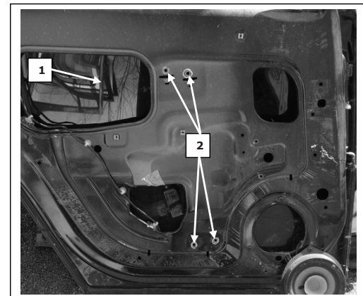
Porta lato sinistro, Portière arrière gauche, Left rear door, Puerta lado izquierdo, Hinten links Tür, Porta traseira esquerda, Sol arka kapi, πόρτα οπισθία αριστερή
