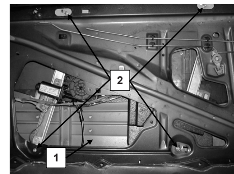
Porta lato destro, Portière avant droite, Right front door, Puerta lado derecho, Vorne rechte Tür, Porta frente dijeta, Sag on kapı, πόρτα εμπρός/δεξιά
