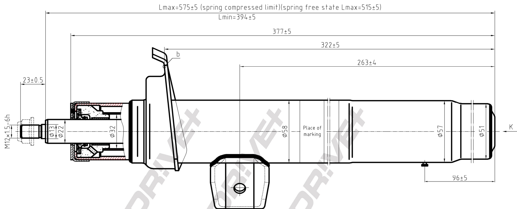
View K Remove spring seat
