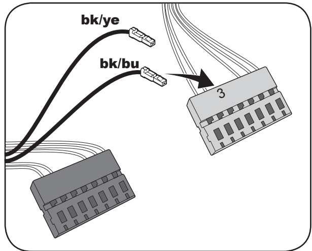
bk/bu → PIN 3 E-Satz Stecker bk/bu → PIN 3 e-kit connector
