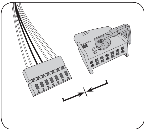
bk/ye → PIN 4 E-Satz Stecker bk/ye → PIN 4 e-kit connector
