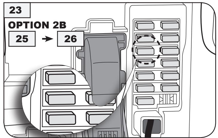
belegt Kammer 3 occupied fuseslot 3
