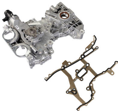
Control housing cover with integrated oil and water pump
