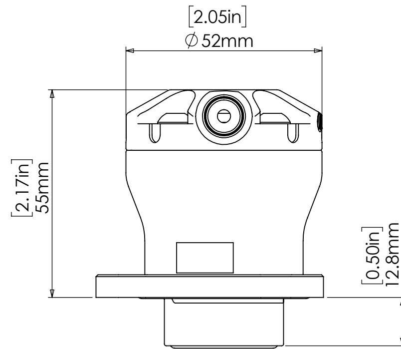
Adjustable Swivel Flange
