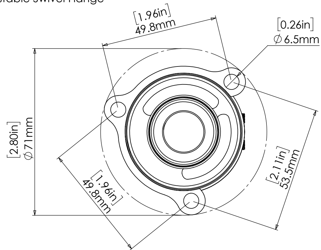
Adjustable Swivel Flange
