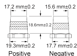
ODP-AGM65 LEFT POSITIVE SAE TERMINALS
