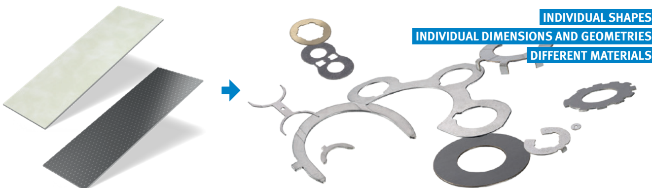
Examples of individual thrust washers, half-washers and other designs made from KS PERMAGLIDE® strips
