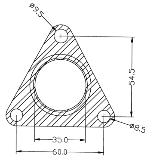
Gasket dimensions
