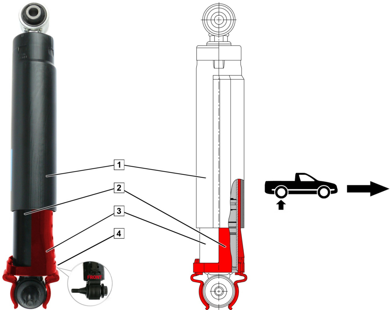
Fig. 1: Shock absorber with additional protection sleeve
