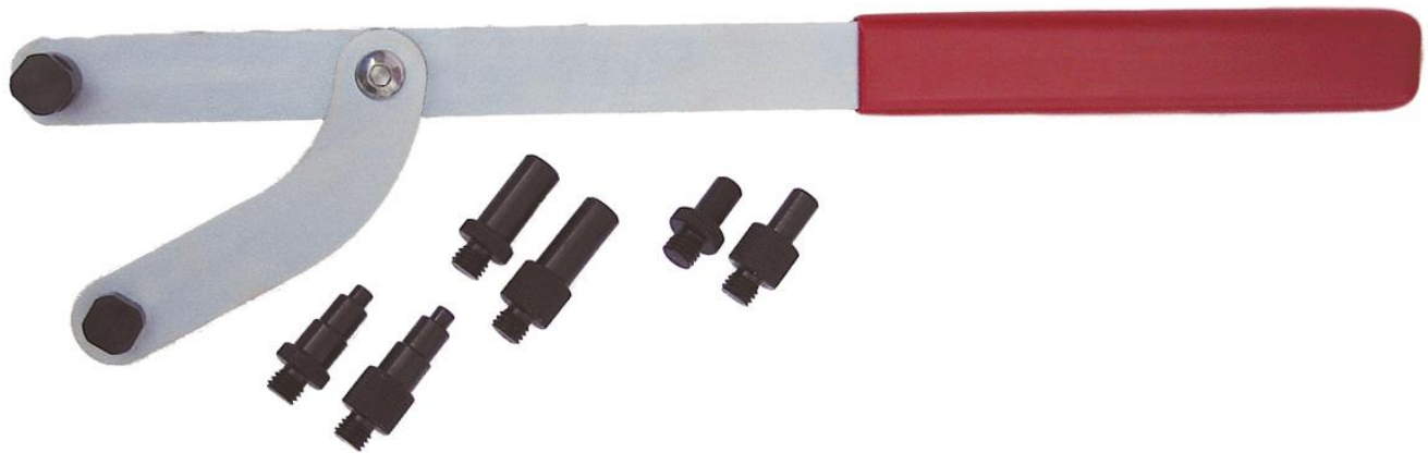
7468-10022 – GAT4844 – Universal Camshaft Sprocket Holding Tool with Interchangeable Pins
