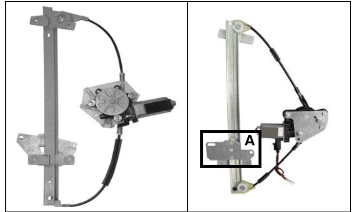
Elevavidros original – lève-vitre original – oem window regulator – levandator de vidro original
