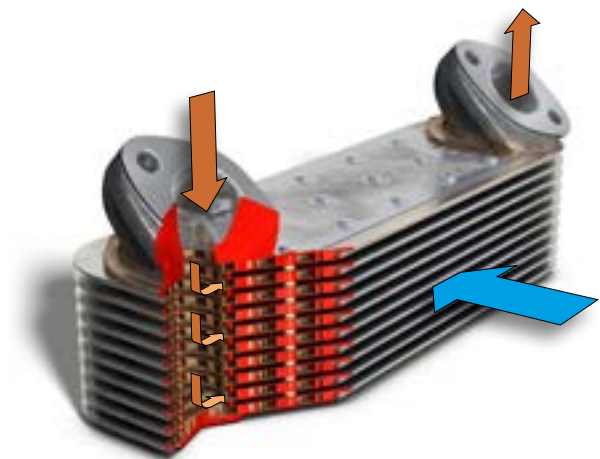
Oil cooler in a utility vehicle
