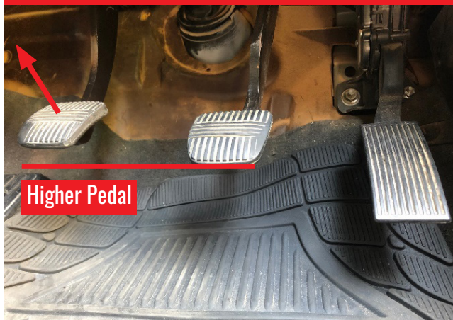
PEDAL BEFORE ADJUSTMENT
