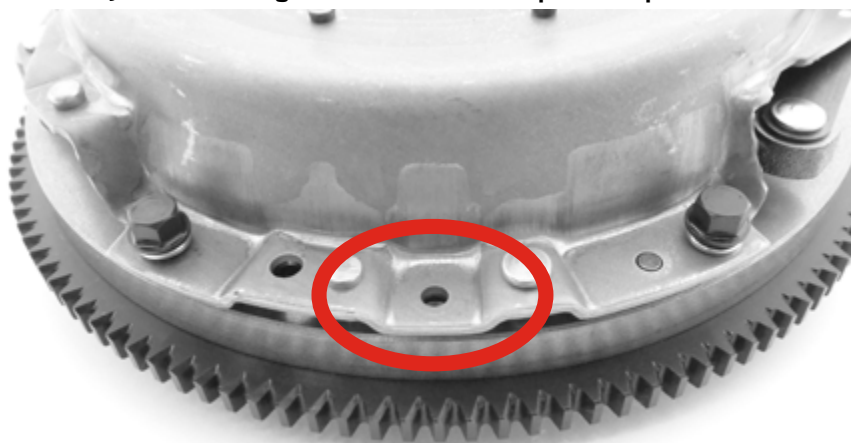
Flywheel showing 3 available holes for pressure plate bolts.
