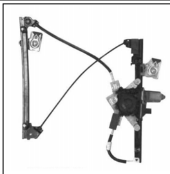
Elevallunas original Oem window regulator
