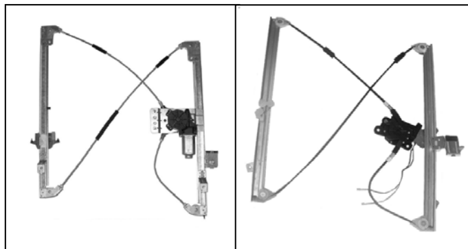
Elevalunas original Oem window regulator
