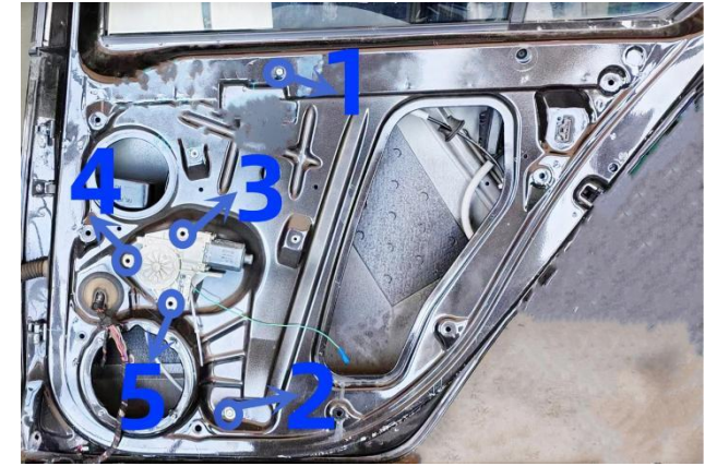
Rear Right
