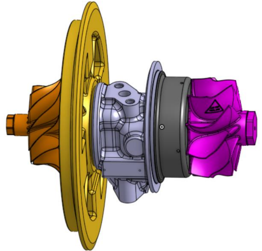
CHRA (Center Housing & Rotating assembly) PN 754190-0152
