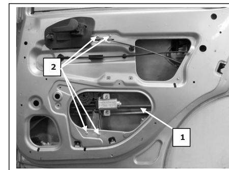
Porta lato destro, Portière arrière droite, Right rear door, Puerta lado derecho, Hinten rechte Tür, Porta traseira direita, Sag arka kapı, νότρο οπίσθια δεξιά
