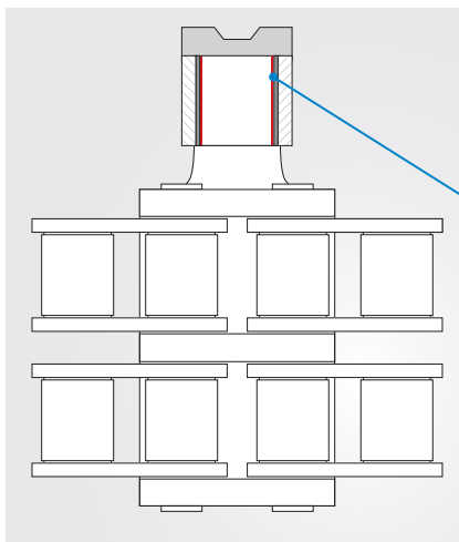
Bearings in cleated chains on high bay lift trucks with KS Permaglide® plain bearing bushes, type PAP ... P200
