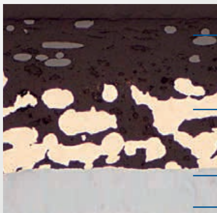
Fig. 1: Microsection of P203
