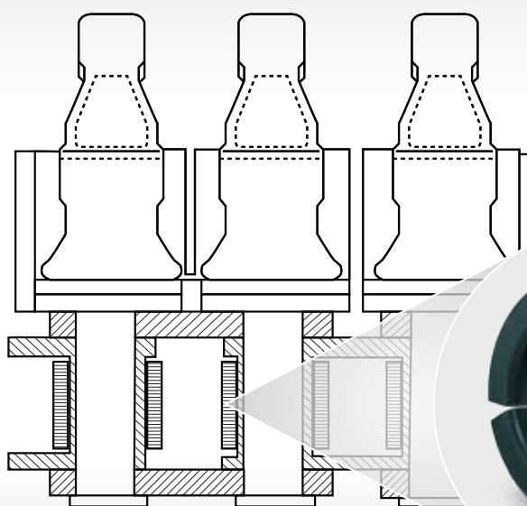
Bearing of the grippers with KS PERMAGLIDE® P10 plain bearing flange bushes
