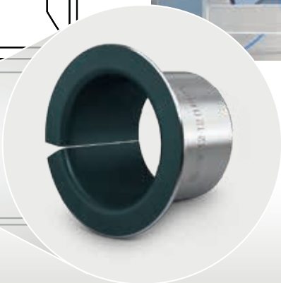
Bearing of the grippers with KS PERMAGLIDE® P10 plain bearing flange bushes
