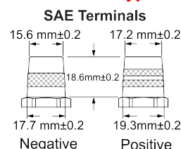
ODP-AGM49/H8/L5 RIGHT POSITIVE SAE TERMINALS
