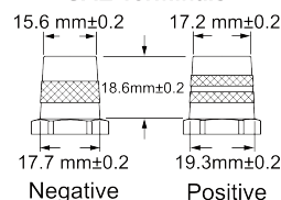
ODP-AGM94R/H7/L4 RIGHT POSITIVE SAE TERMINALS
